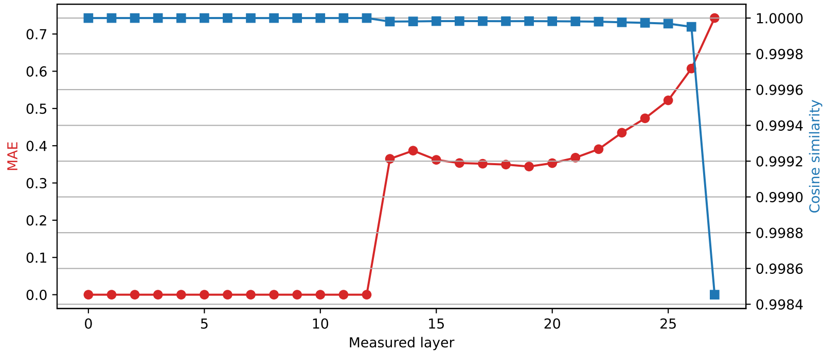
Qwen2.5-7B-Instruct | Quantized layer 12 | float16 → int4
