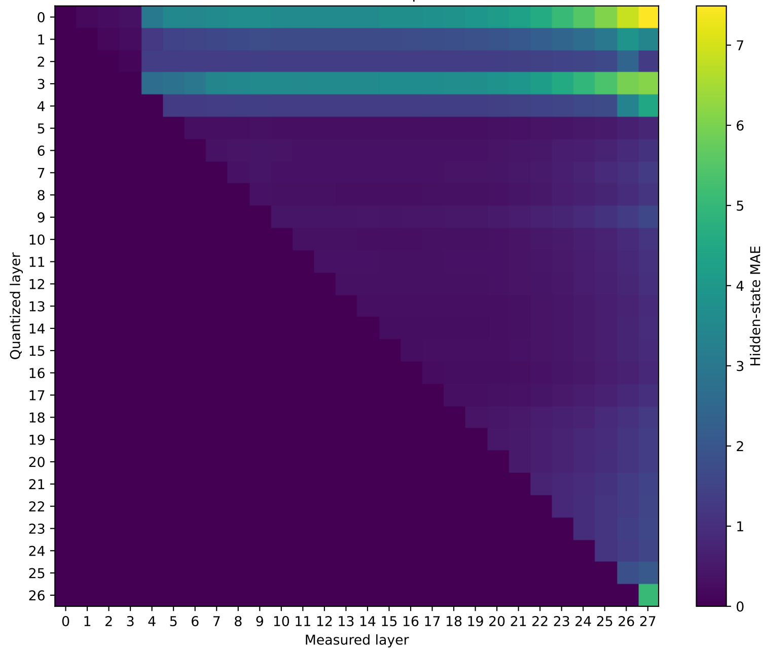
Model: Qwen2.5-7B-Instruct | float16 → int2
