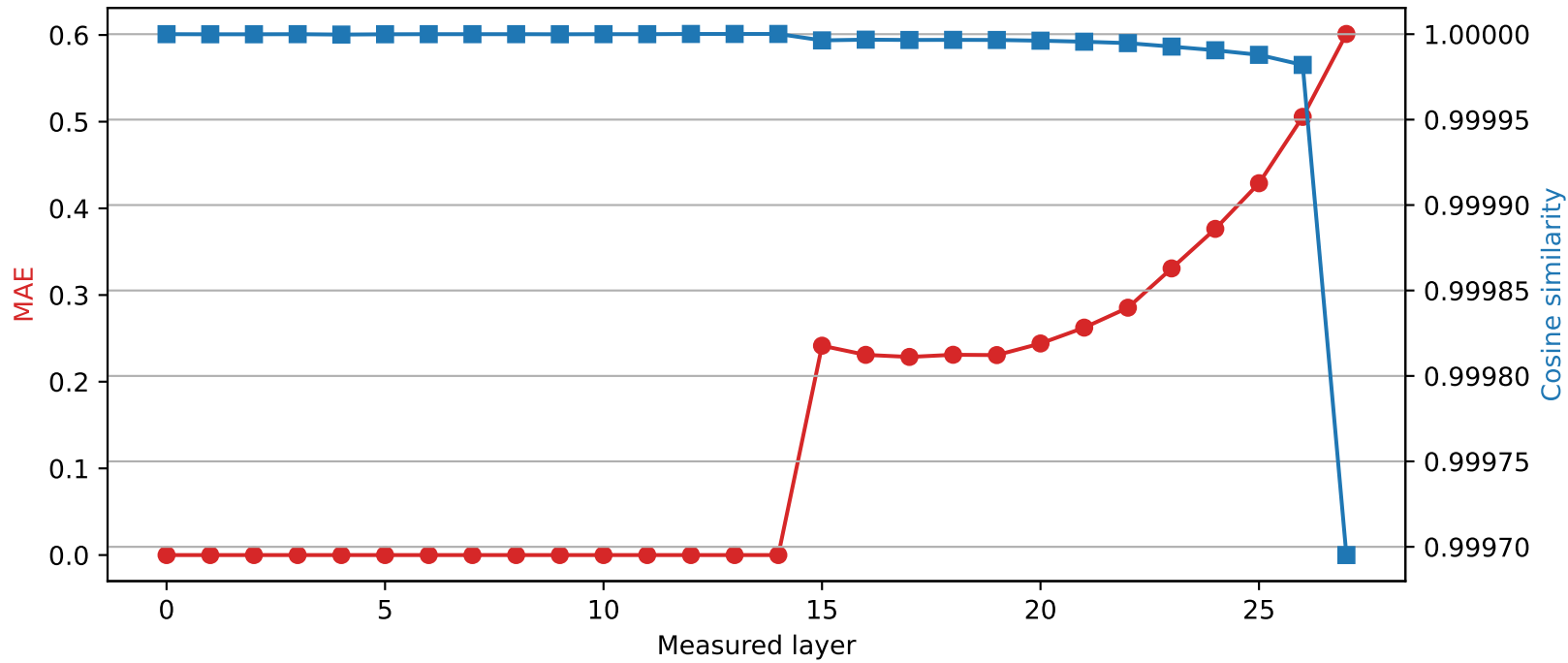
Qwen2.5-7B-Instruct | Quantized layer 14 | float16 \rightarrow int2
