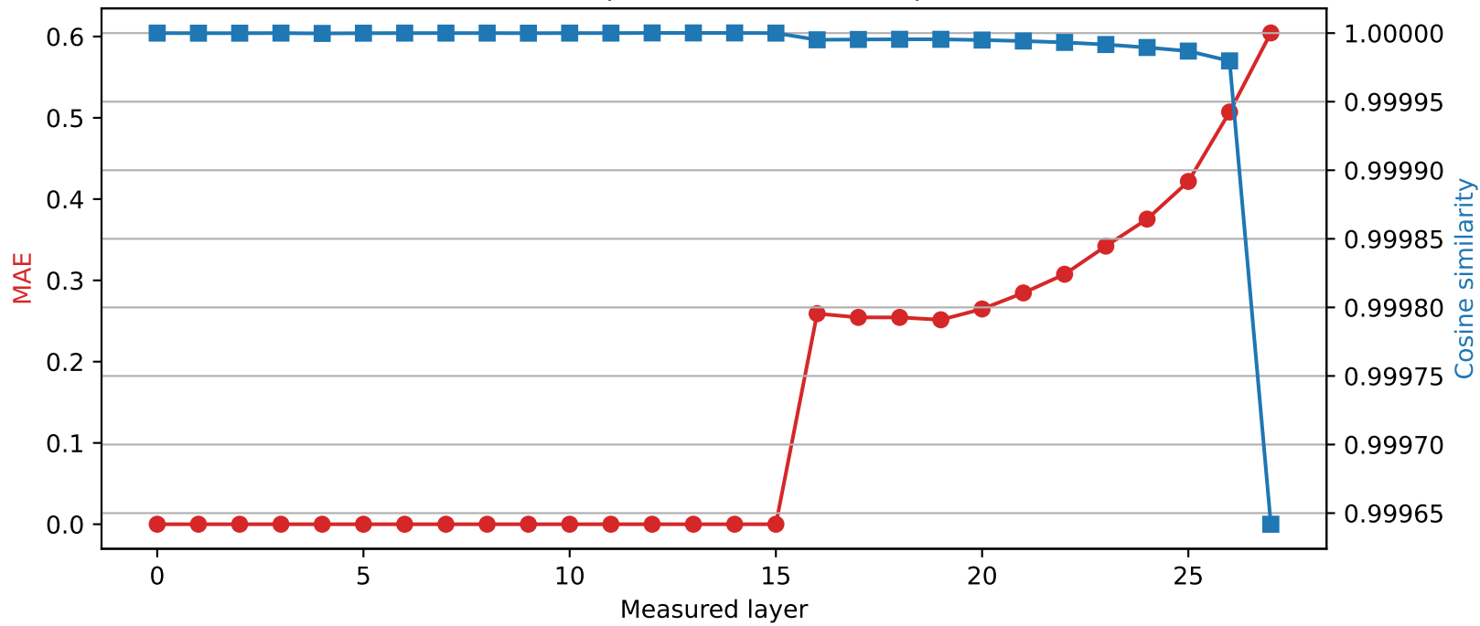
Qwen2.5-7B-Instruct | Quantized layer 15 | float16 \rightarrow int2
