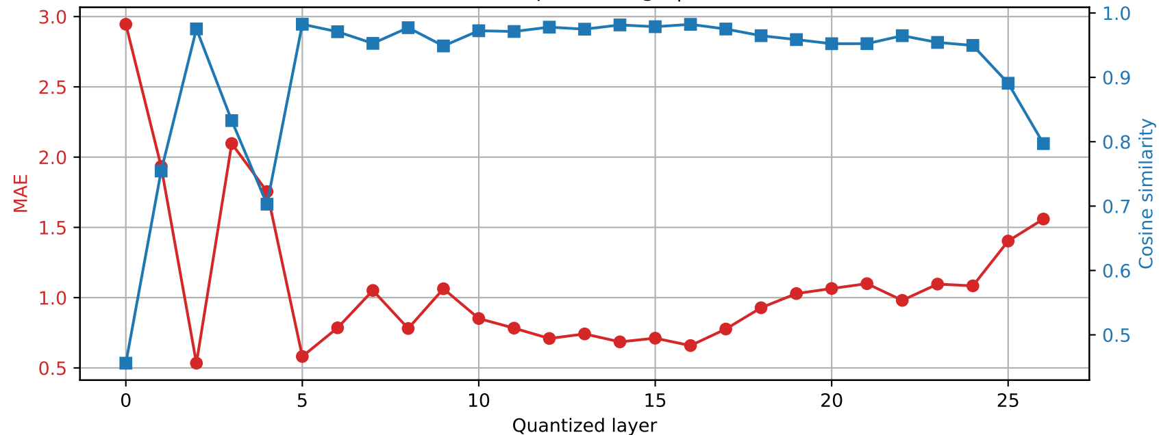
Qwen2.5-7B-Instruct | Prompt 1 Final RMSNorm output damage | float16 \rightarrow int2
