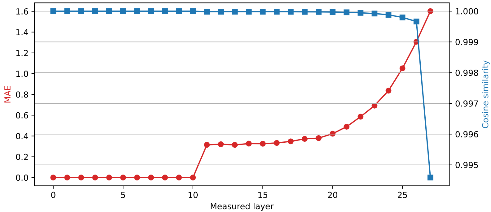
Qwen2.5-7B-Instruct | Quantized layer 10 | float16 \rightarrow int2
