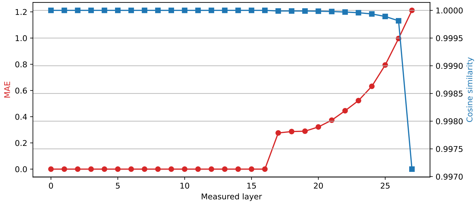
Qwen2.5-7B-Instruct | Quantized layer 16 | float16 \rightarrow int2
