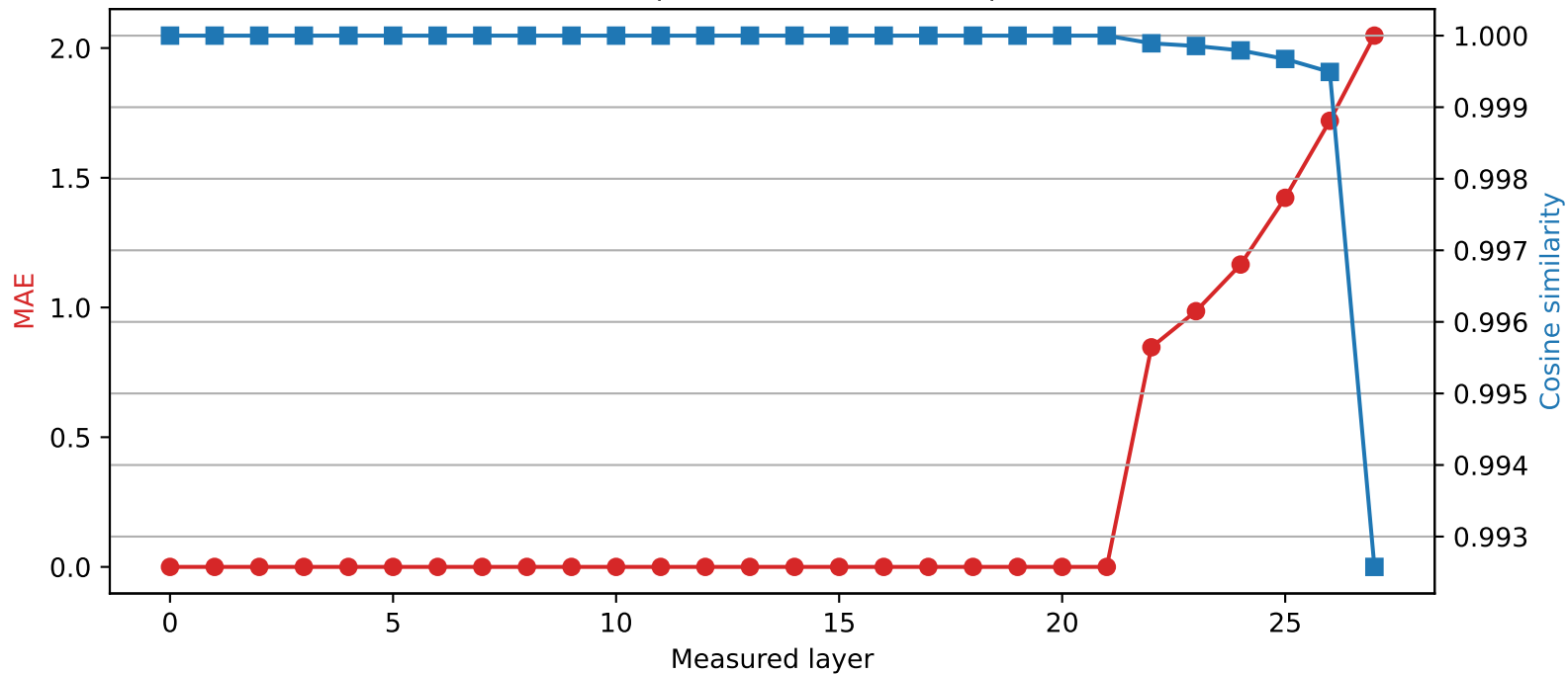
Qwen2.5-7B-Instruct | Quantized layer 21 | float16 → int2
