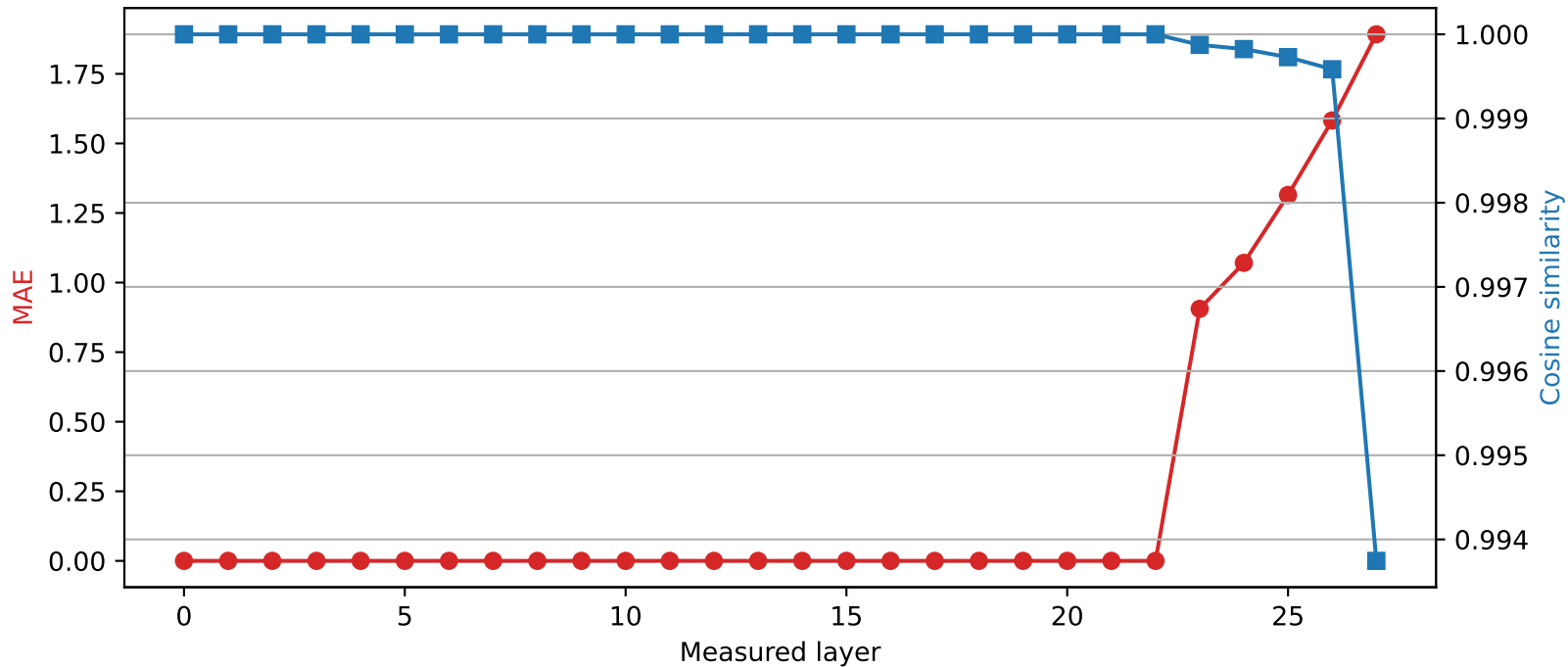
Qwen2.5-7B-Instruct | Quantized layer 22 | float16 → int2
