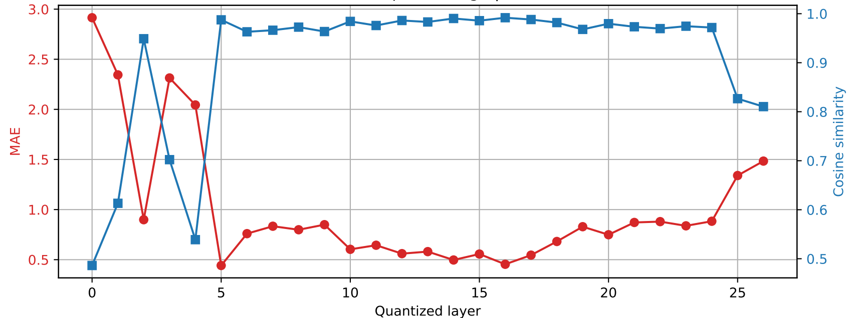
Qwen2.5-7B-Instruct | Prompt 2 Final RMSNorm output damage | float16 \rightarrow int2
