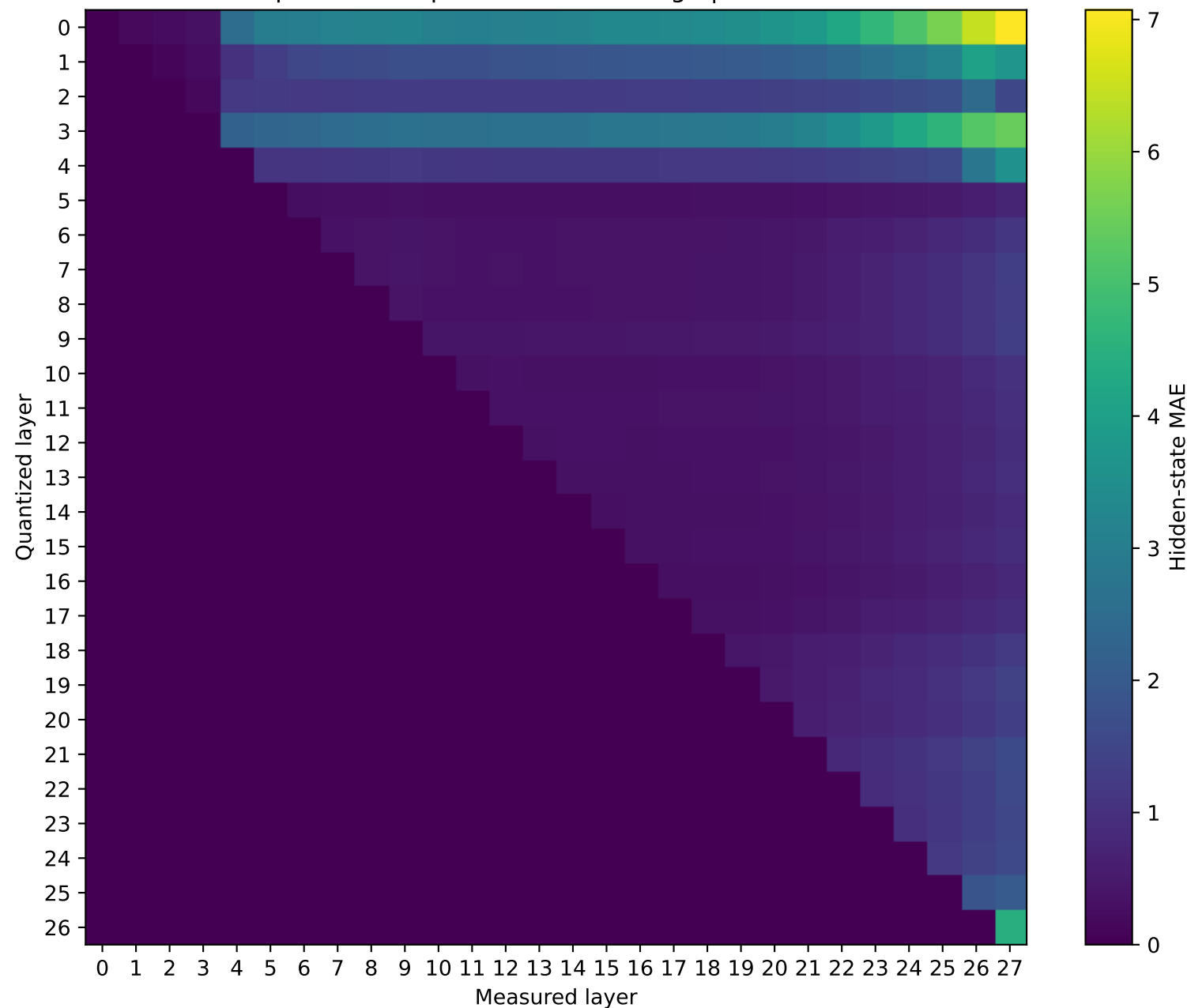
Qwen2.5-7B-Instruct Prompt 2: MAE representation damage | float16 \rightarrow int2
