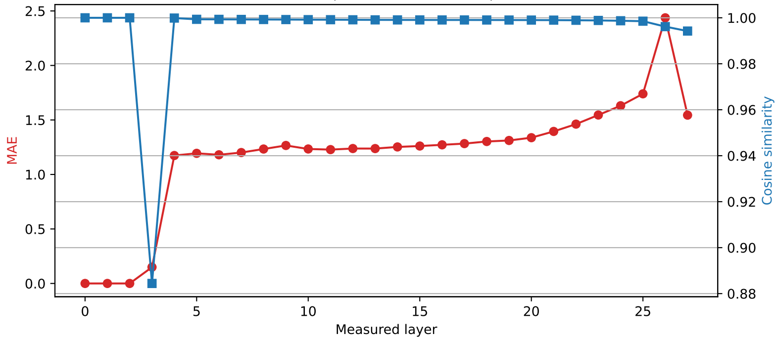
Qwen2.5-7B-Instruct | Quantized layer 2 | float16 \rightarrow int2
