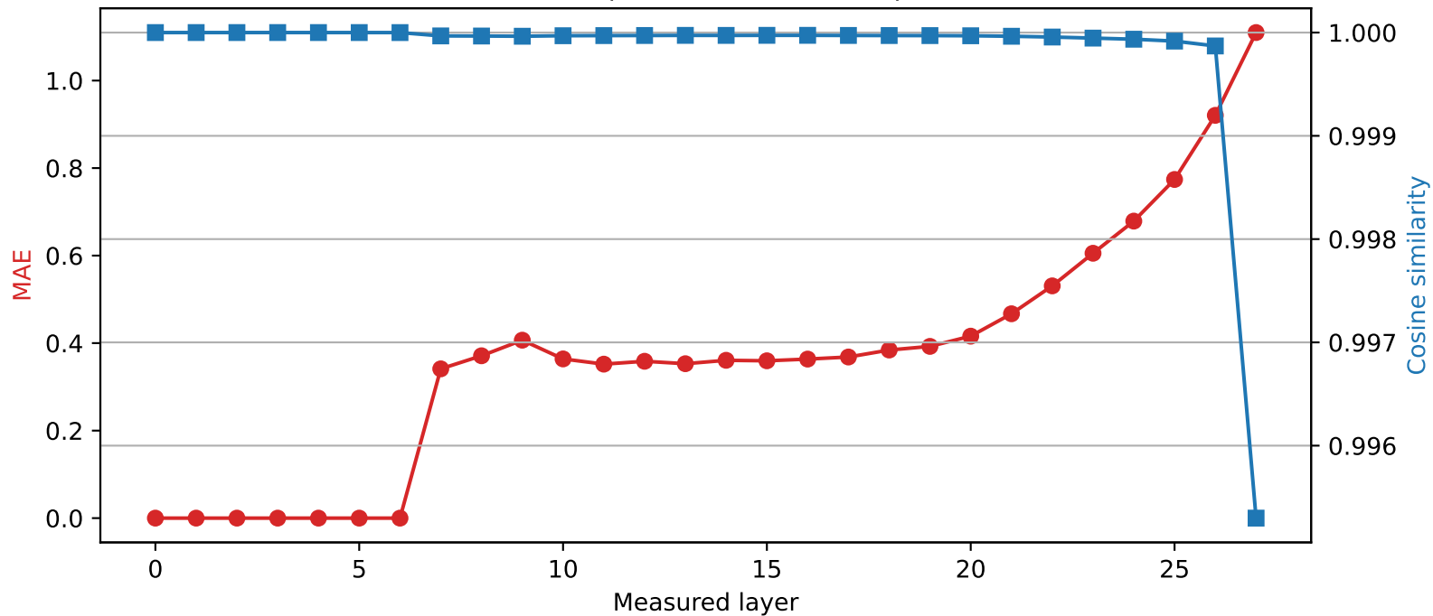
Qwen2.5-7B-Instruct | Quantized layer 6 | float16 \rightarrow int2
