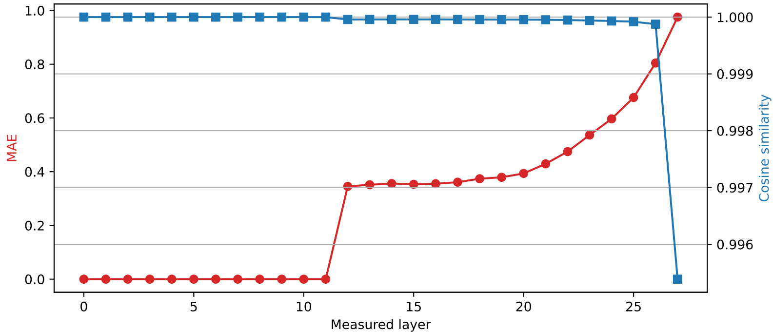
Qwen2.5-7B-Instruct | Quantized layer 11 | float16 \rightarrow int2
