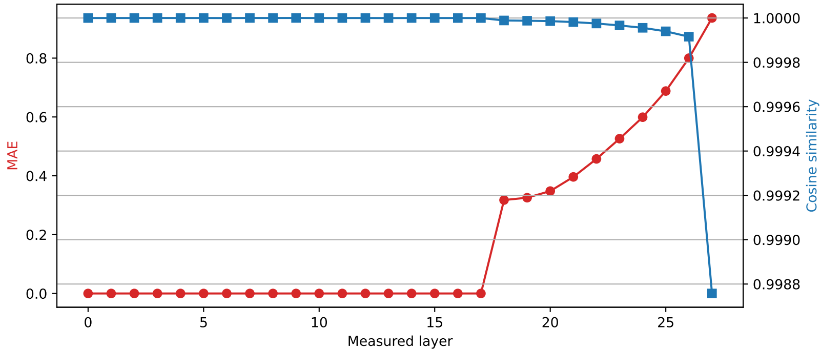
Qwen2.5-7B-Instruct | Quantized layer 17 | float16 \rightarrow int2
