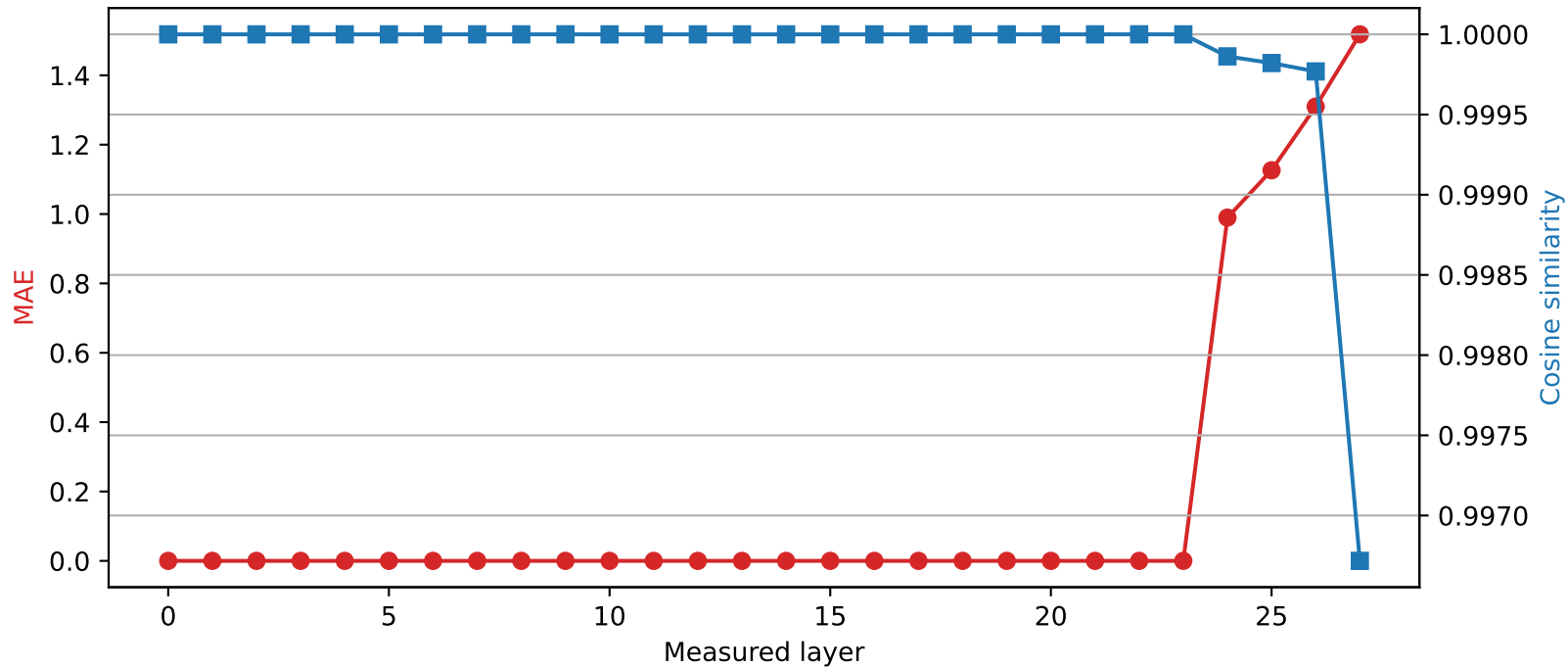
Qwen2.5-7B-Instruct | Quantized layer 23 | float16 → int2
