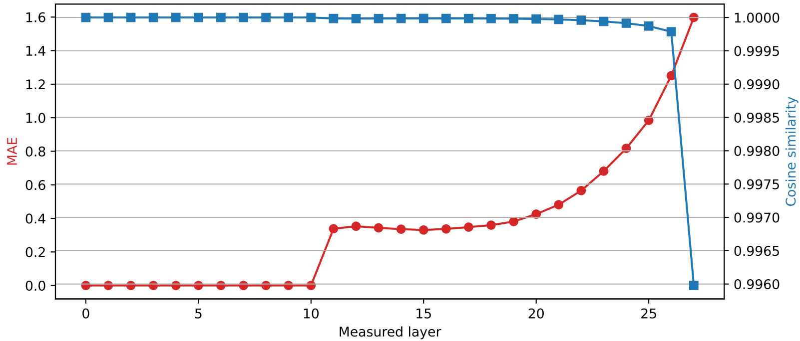
Qwen2.5-7B-Instruct | Quantized layer 10 | float16 → int2
