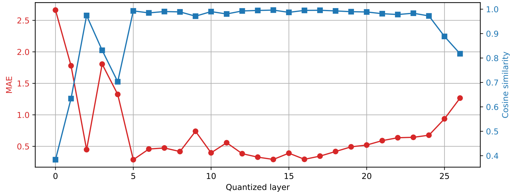
Qwen2.5-7B-Instruct | Prompt 4 Final RMSNorm output damage | float16 \rightarrow int2
