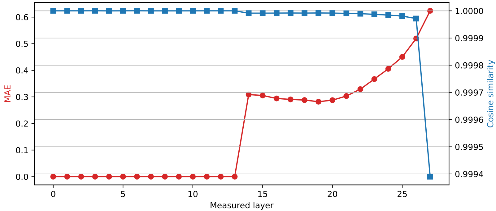
Qwen2.5-7B-Instruct | Quantized layer 13 | float16 \rightarrow int2
