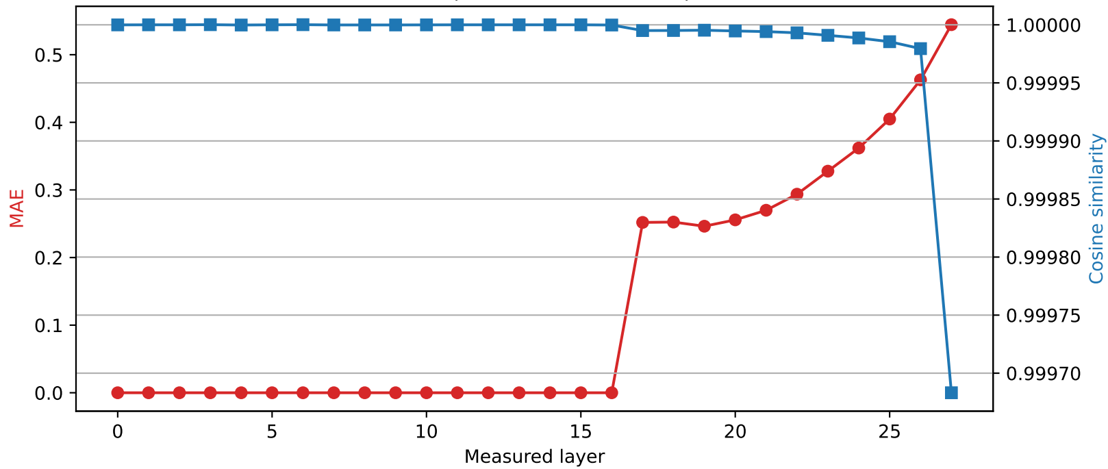
Qwen2.5-7B-Instruct | Quantized layer 16 | float16 → int2
