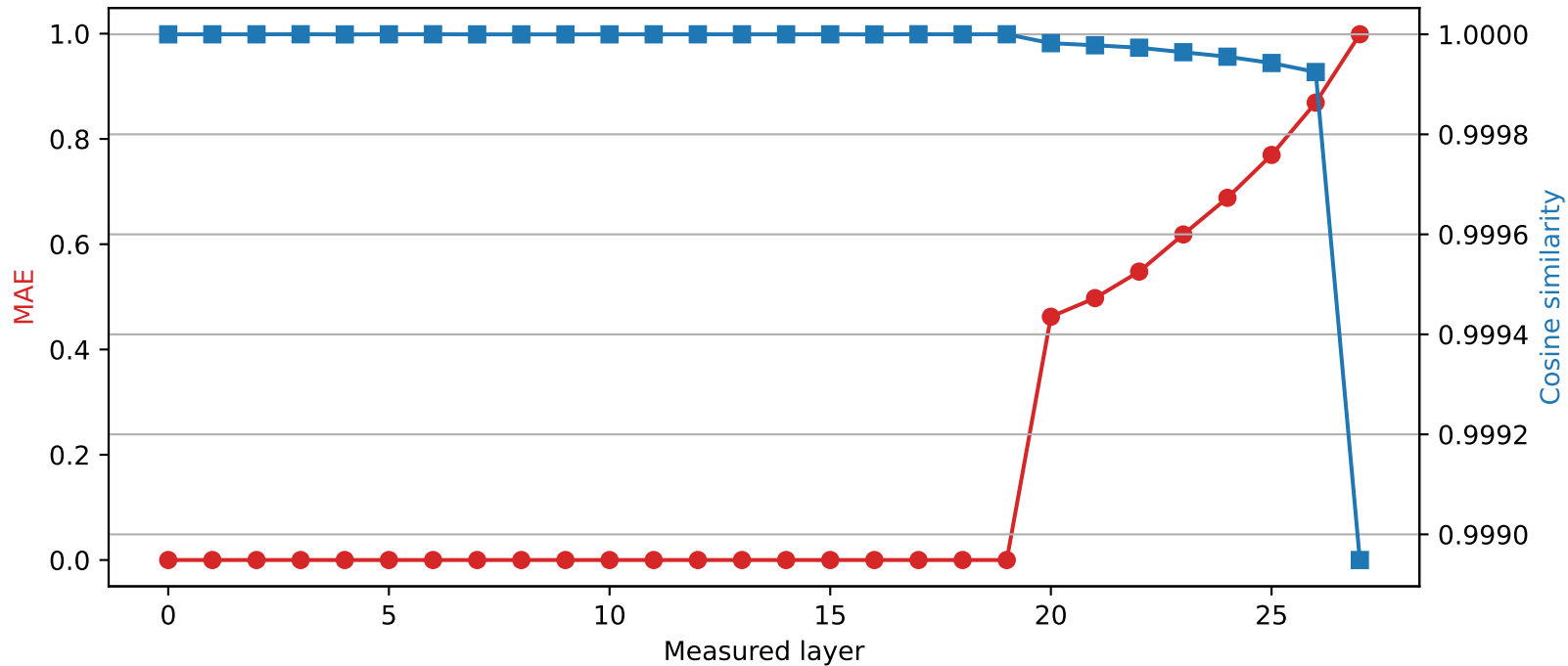
Qwen2.5-7B-Instruct | Quantized layer 19 | float16 \rightarrow int2
