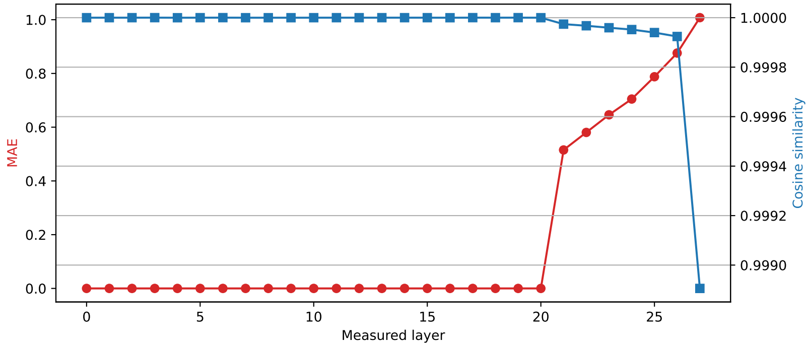
Qwen2.5-7B-Instruct | Quantized layer 20 | float16 → int2
