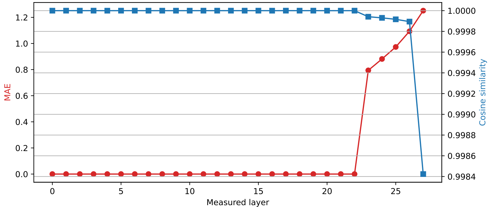
Qwen2.5-7B-Instruct | Quantized layer 22 | float16 \rightarrow int2
