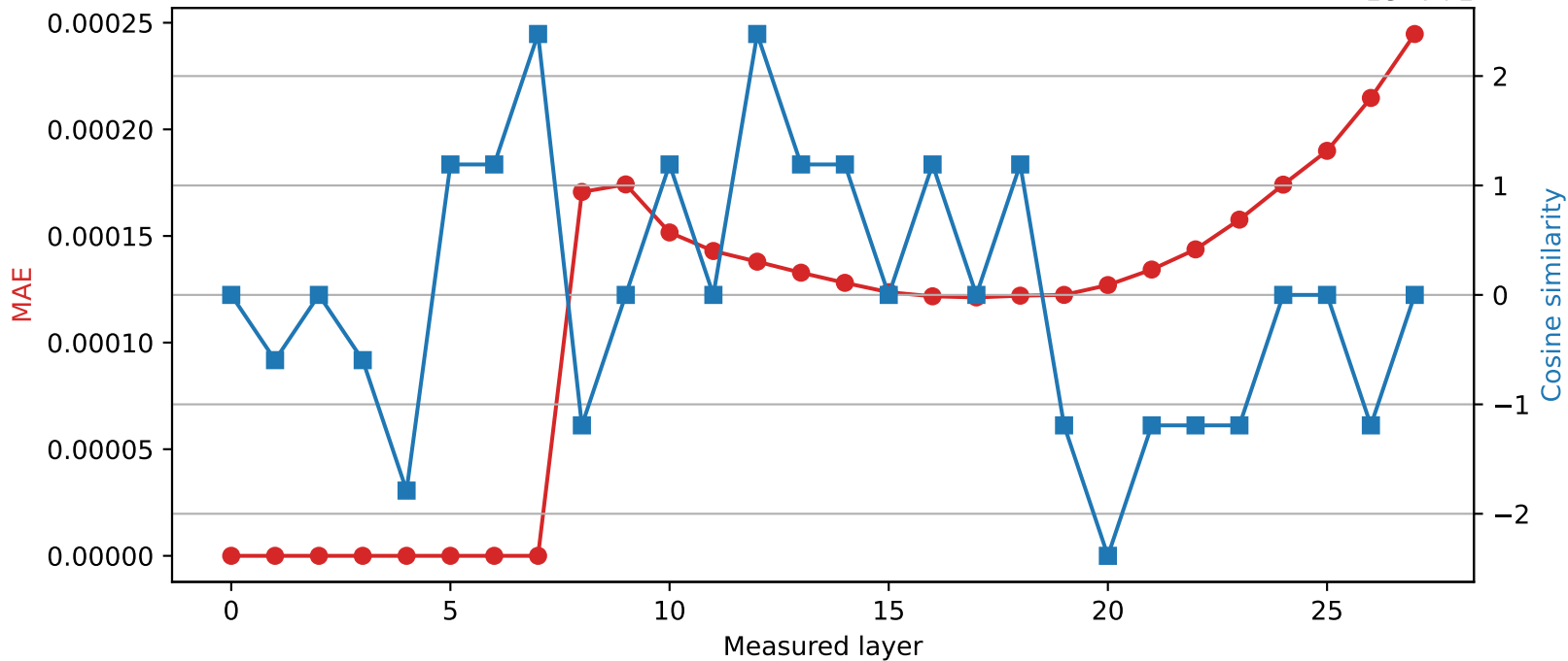
Qwen2.5-7B-Instruct | Quantized layer 7 | float32 → int16
