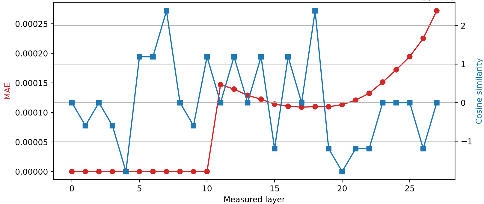
Qwen2.5-7B-Instruct | Quantized layer 10 | float32 \rightarrow int16
