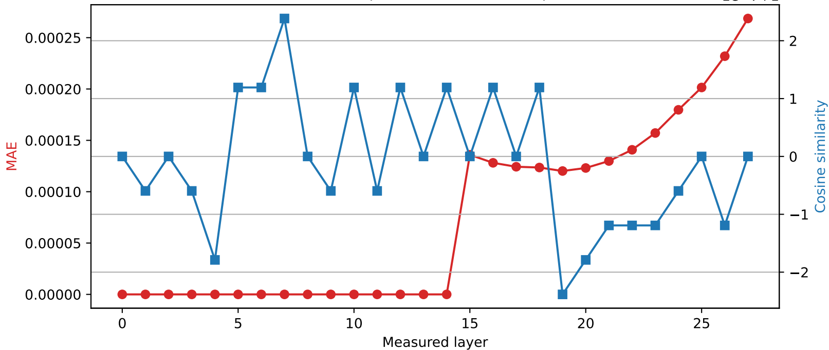
Qwen2.5-7B-Instruct | Quantized layer 14 | float32 \rightarrow int16
