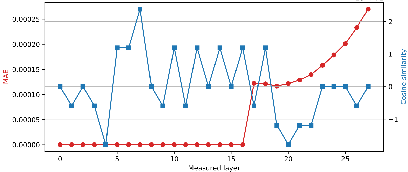
Qwen2.5-7B-Instruct | Quantized layer 16 | float32 \rightarrow int16
