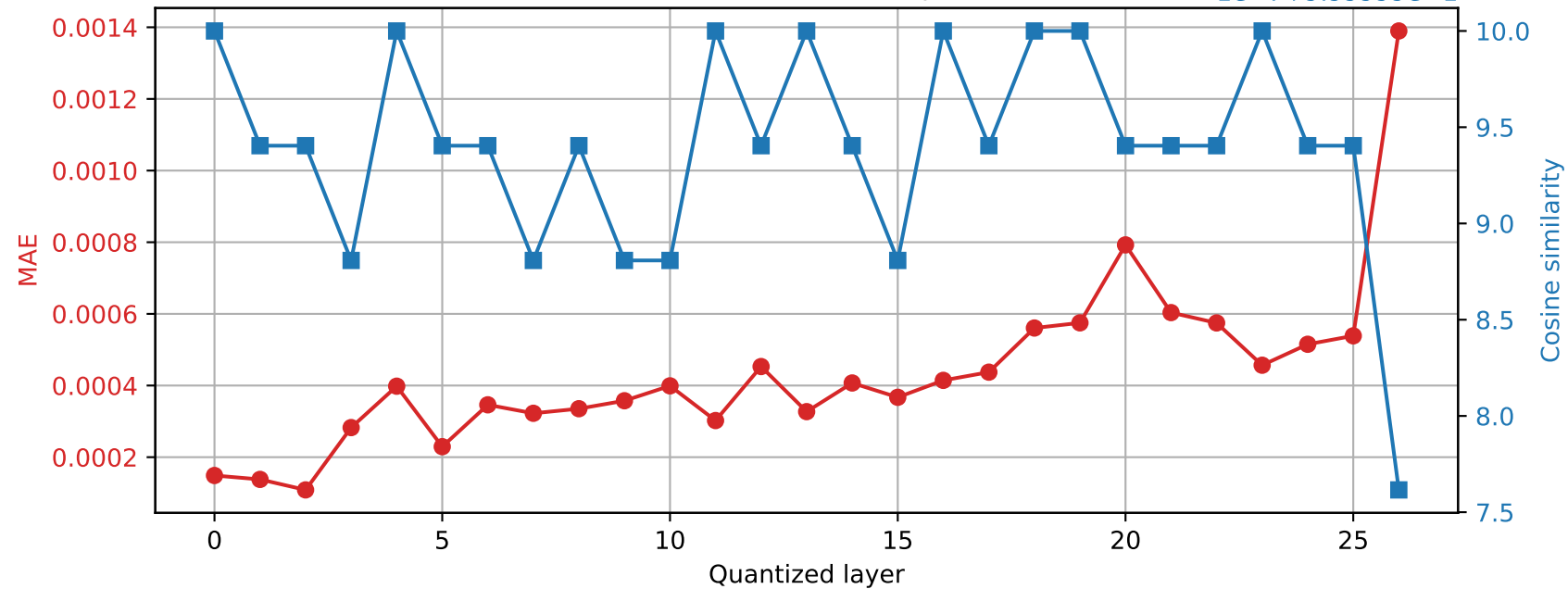
Qwen2.5-7B-Instruct | Prompt 1 Final RMSNorm output damage | float32 \rightarrow int16
