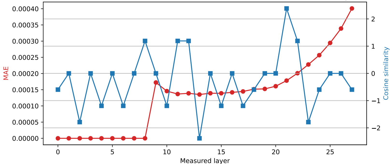
Qwen2.5-7B-Instruct | Quantized layer 8 | float32 \rightarrow int16
