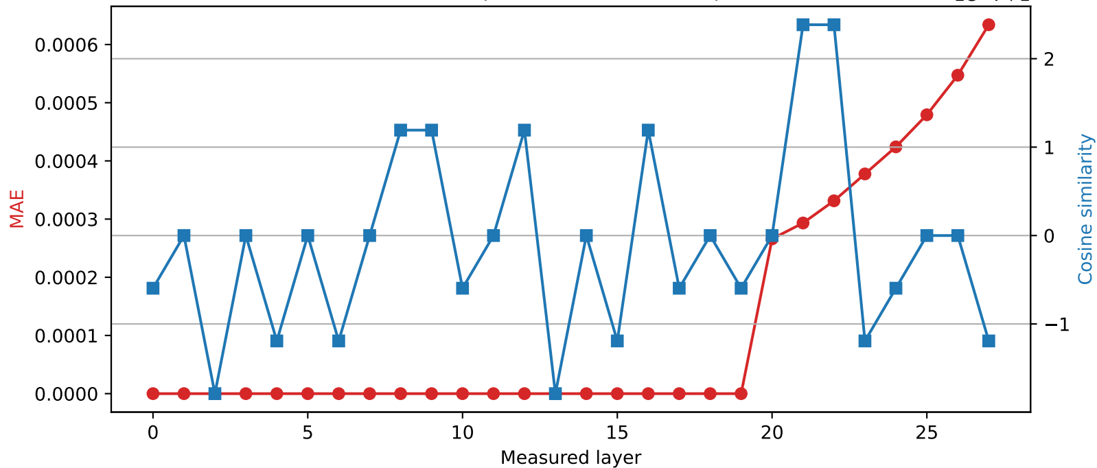
Qwen2.5-7B-Instruct | Quantized layer 19 | float32 \rightarrow int16
