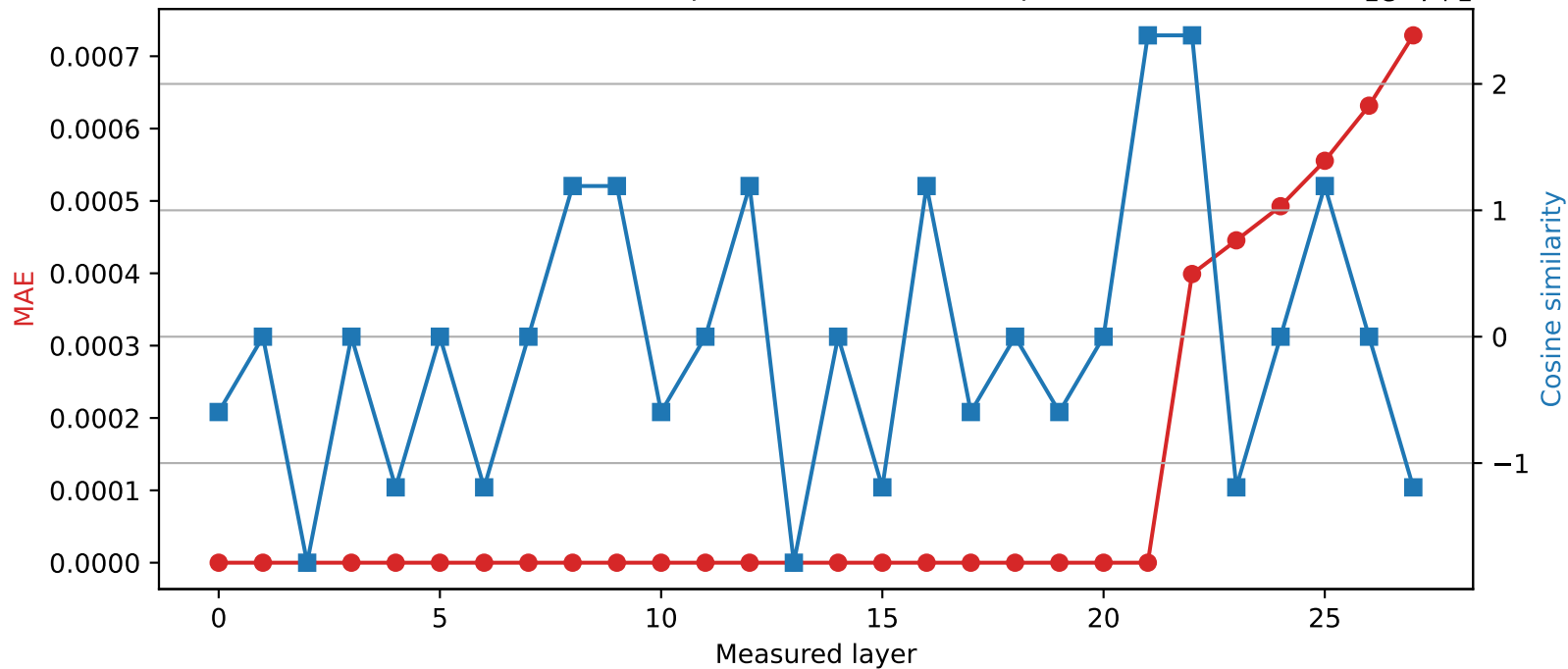
Qwen2.5-7B-Instruct | Quantized layer 21 | float32 \rightarrow int16
