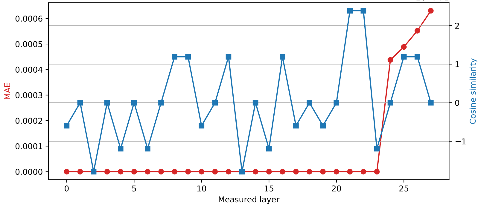
Qwen2.5-7B-Instruct | Quantized layer 23 | float32 \rightarrow int16
