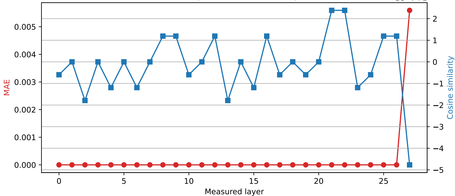
Qwen2.5-7B-Instruct | Quantized layer 26 | float32 \rightarrow int16
