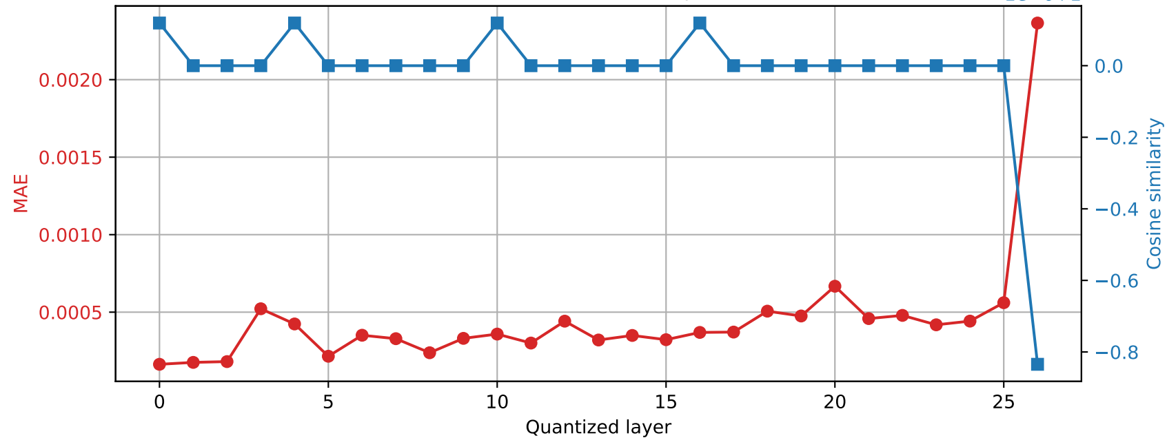
Qwen2.5-7B-Instruct | Prompt 3 Final RMSNorm output damage | float32 → int16
