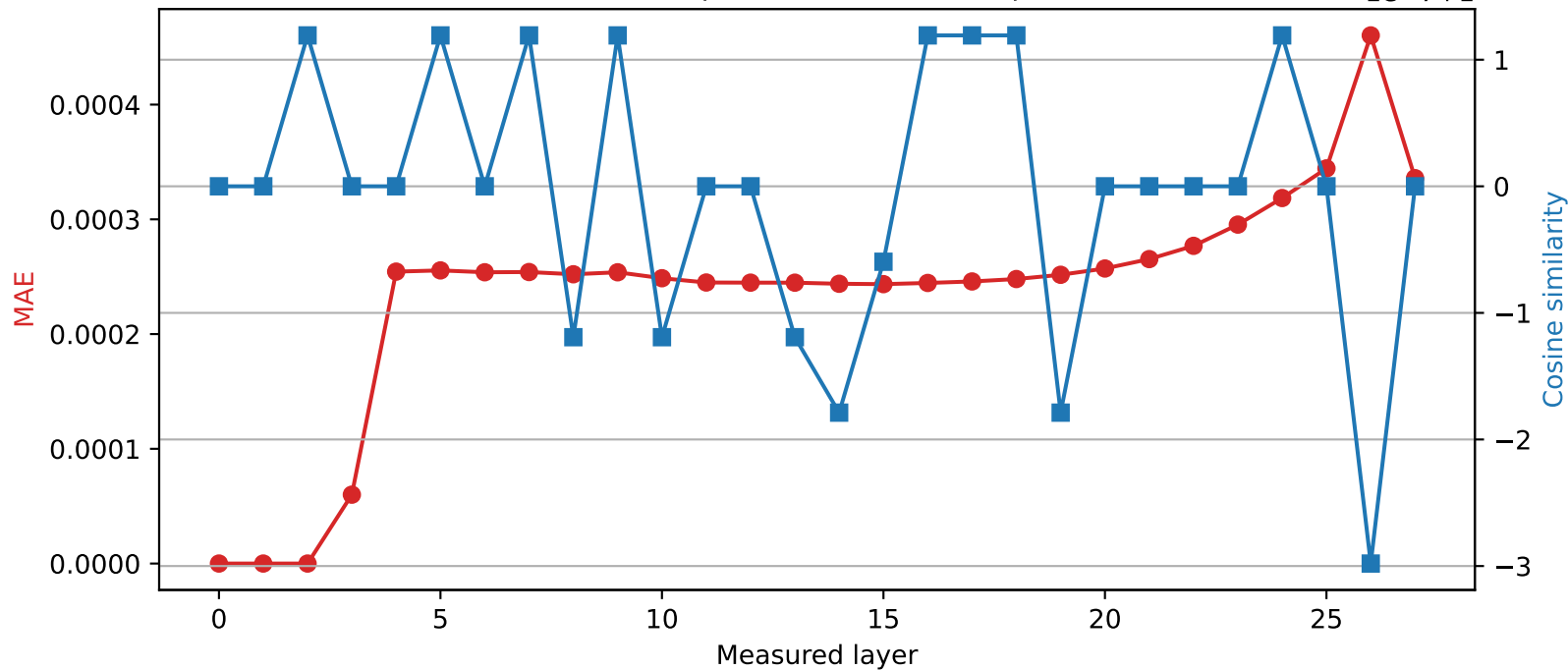
Qwen2.5-7B-Instruct | Quantized layer 2 | float32 → int16
