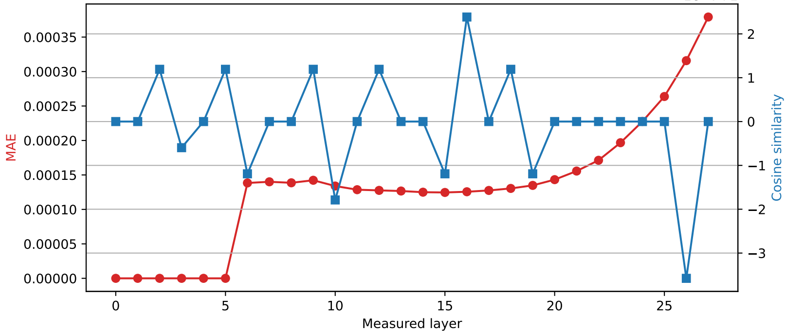
Qwen2.5-7B-Instruct | Quantized layer 5 | float32 → int16
