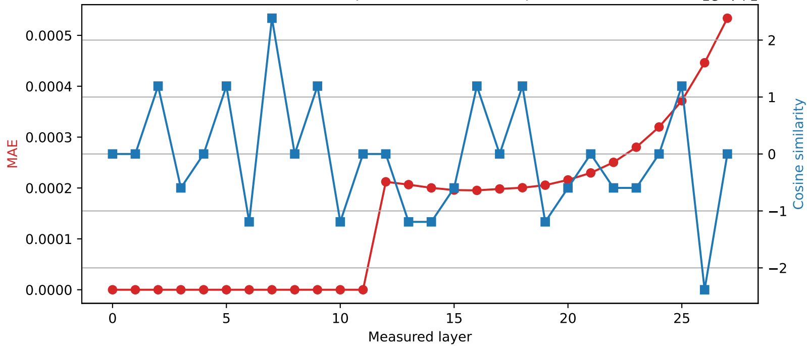
Qwen2.5-7B-Instruct | Quantized layer 11 | float32 \rightarrow int16
