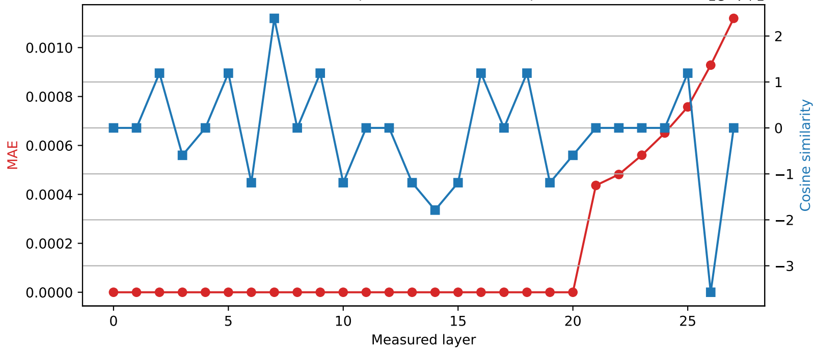
Qwen2.5-7B-Instruct | Quantized layer 20 | float32 \rightarrow int16
