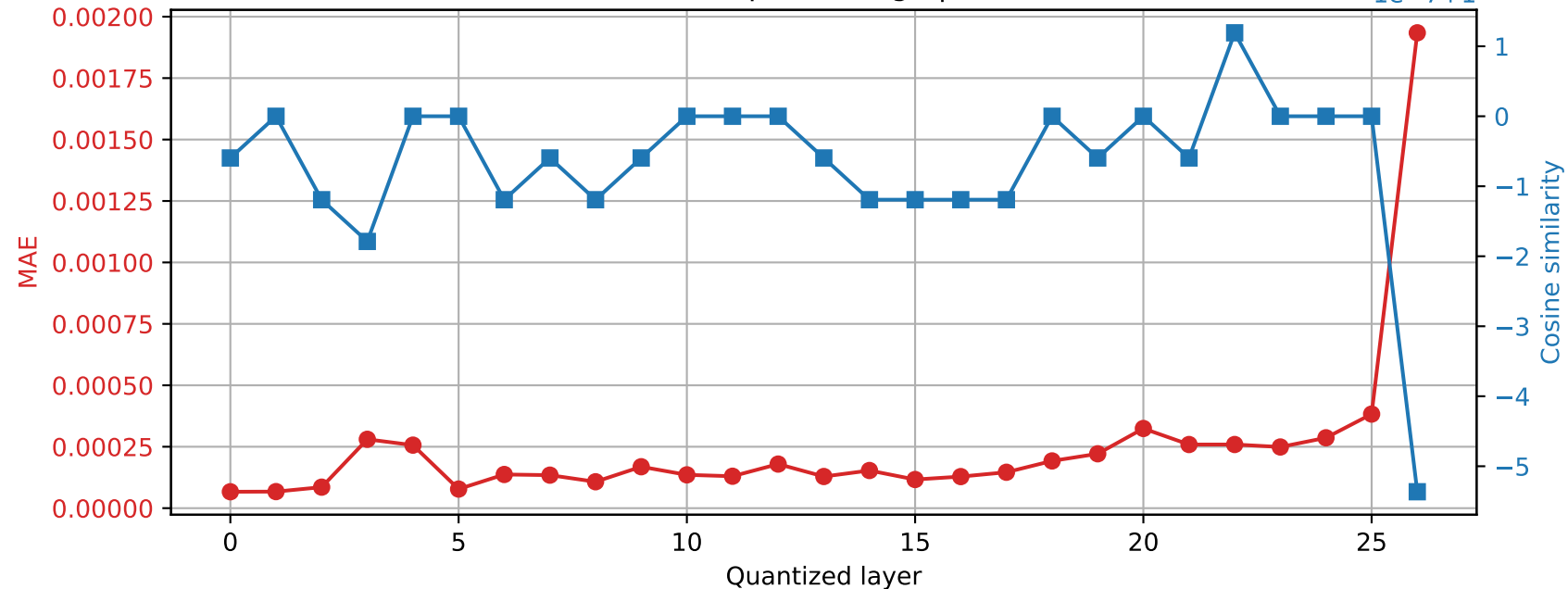
Qwen2.5-7B-Instruct | Prompt 4 Final RMSNorm output damage | float32 \rightarrow int16
