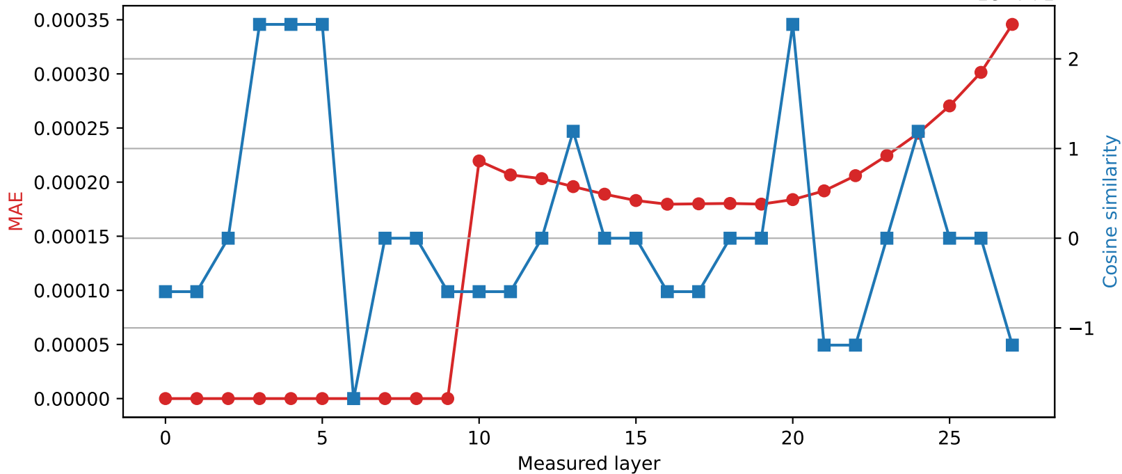
Qwen2.5-7B-Instruct | Quantized layer 9 | float32 → int16
