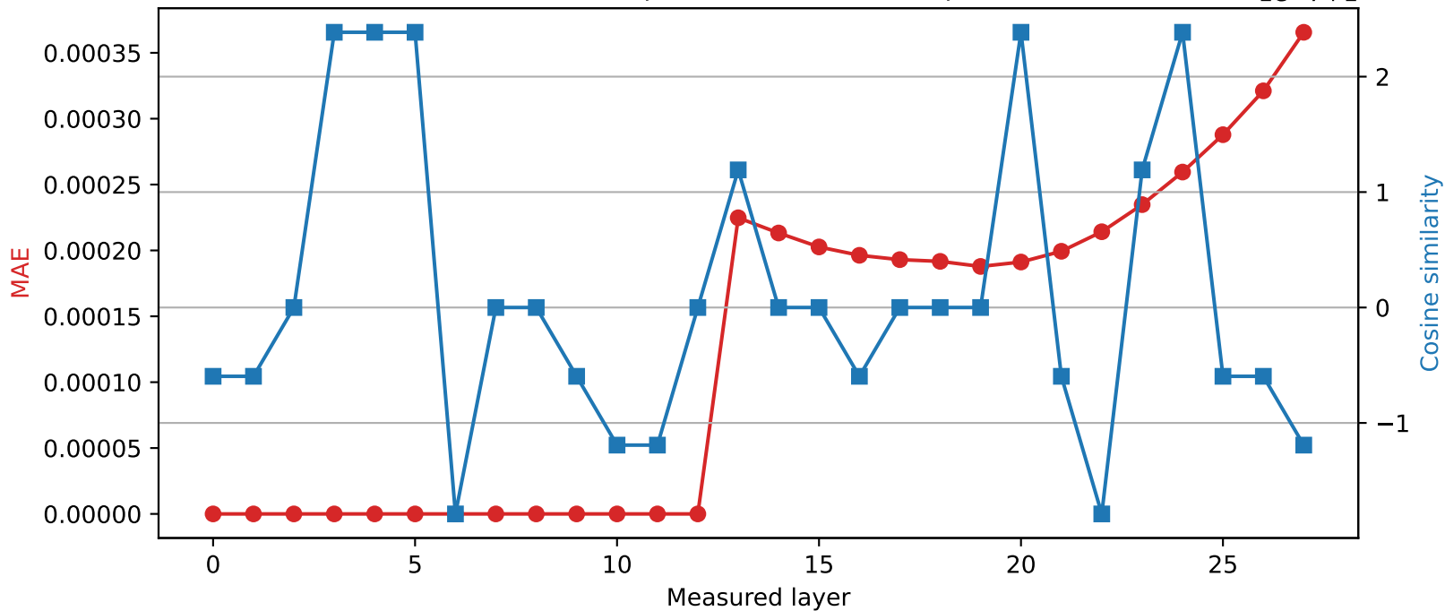
Qwen2.5-7B-Instruct | Quantized layer 12 | float32 \rightarrow int16
