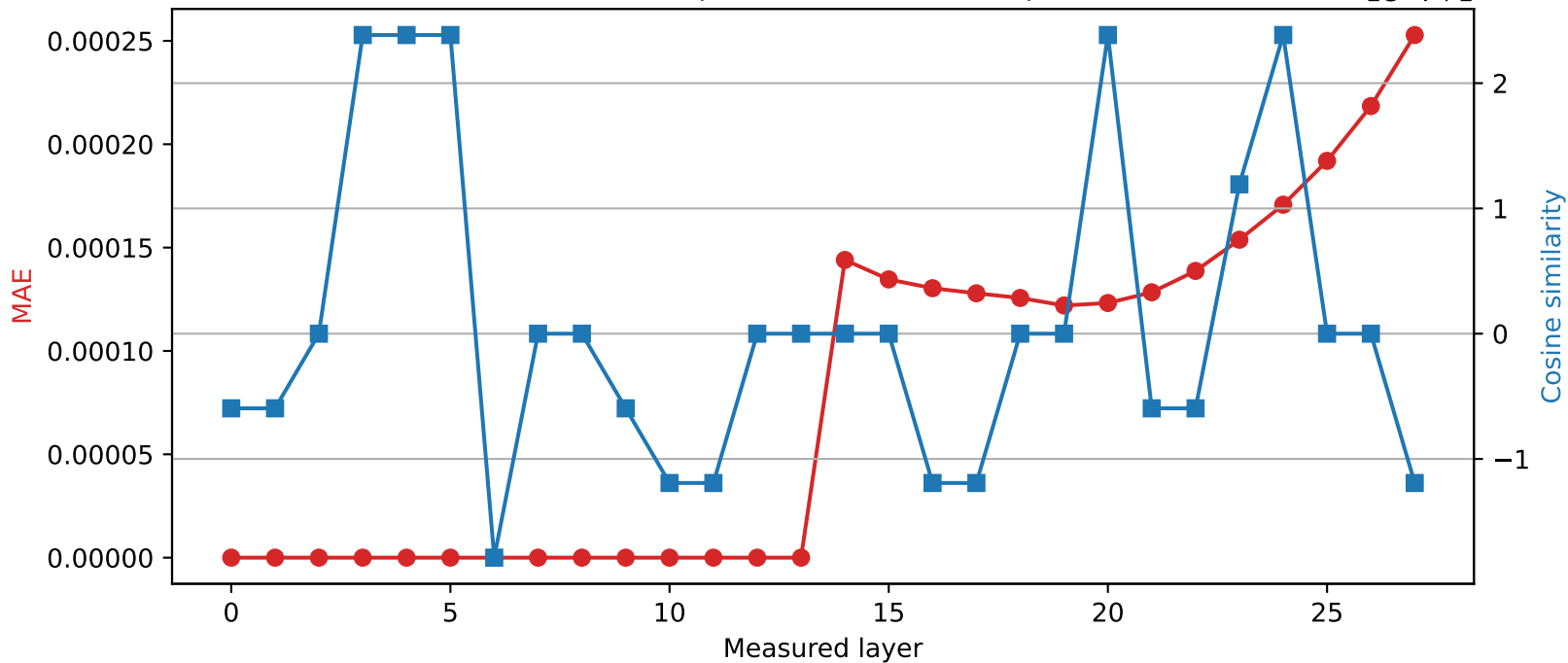
Qwen2.5-7B-Instruct | Quantized layer 13 | float32 \rightarrow int16
