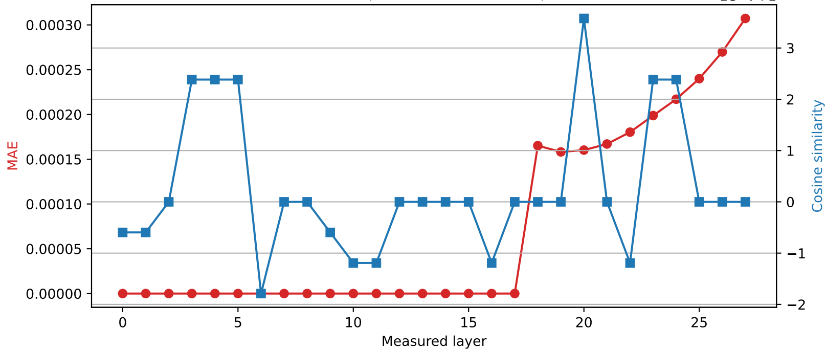
Qwen2.5-7B-Instruct | Quantized layer 17 | float32 \rightarrow int16
