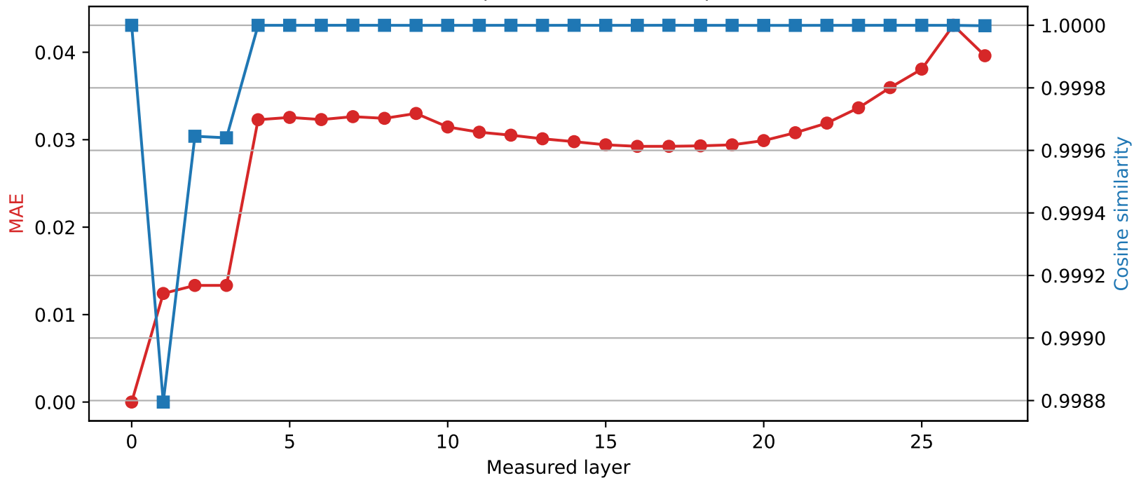
Qwen2.5-7B-Instruct | Quantized layer 0 | float32 → int8
