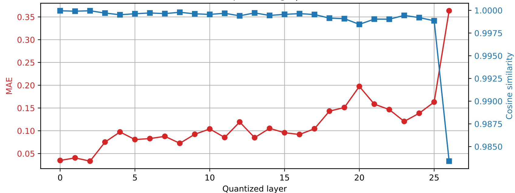
Qwen2.5-7B-Instruct | Prompt 1 Final RMSNorm output damage | float32 → int8
