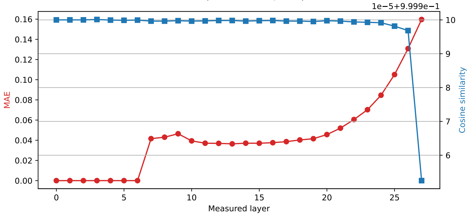
Qwen2.5-7B-Instruct | Quantized layer 6 | float32 → int8
