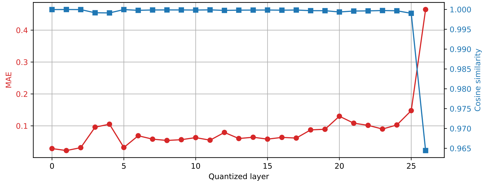
Qwen2.5-7B-Instruct | Prompt 2 Final RMSNorm output damage | float32 → int8
