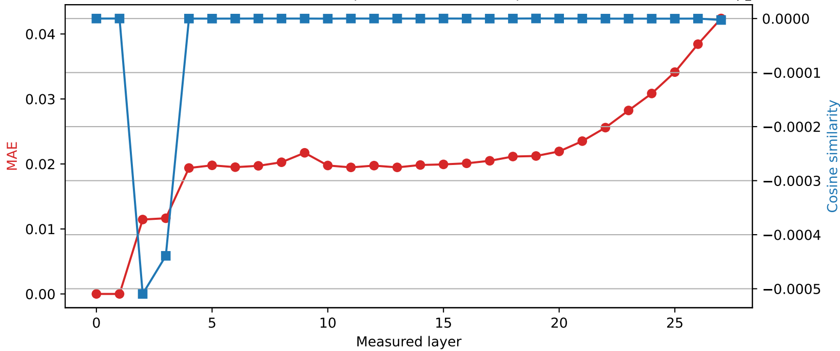
Qwen2.5-7B-Instruct | Quantized layer 1 | float32 \rightarrow int8
