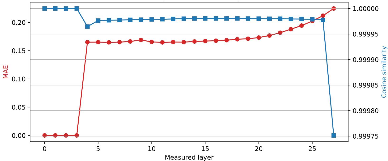
Qwen2.5-7B-Instruct | Quantized layer 3 | float32 → int8
