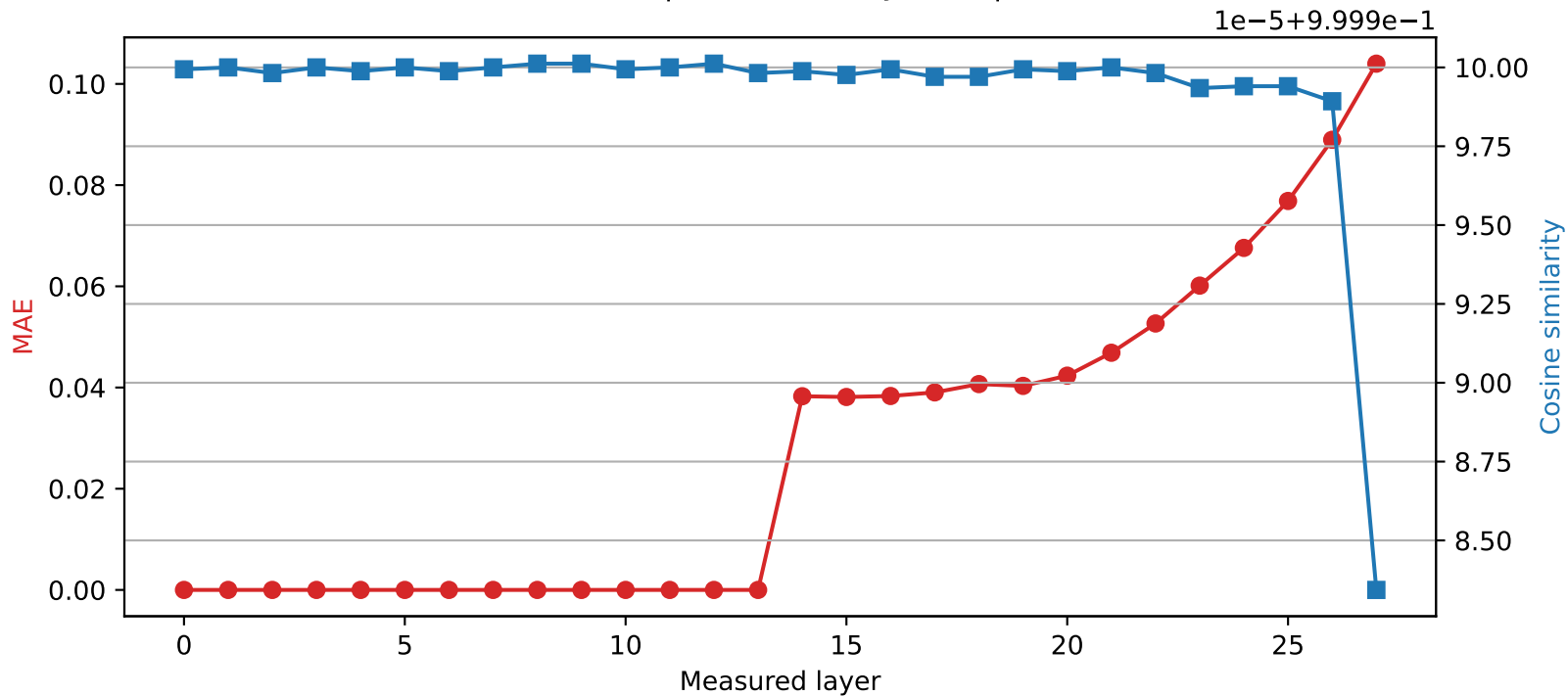
Qwen2.5-7B-Instruct | Quantized layer 13 | float32 → int8
